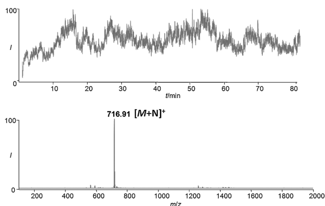
Figure 3. Total ion chronogram of ionized n\text{-C}_{50}\text{H}_{102} and its reaction products recorded on-line. The dominant product is the N-atom insertion product m/z 716 [M+\text{N}]^+ .
